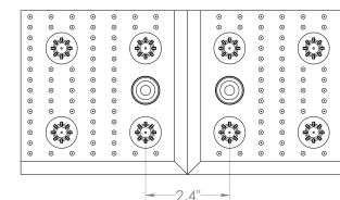
PLAN VIEW: 2-PANELS
